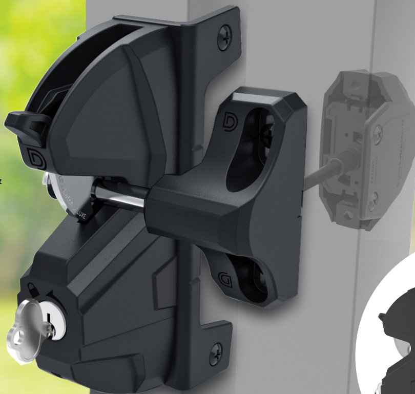
EXTERNAL VIEW EXTERNAL ACCESS BUTTON (EAB)
