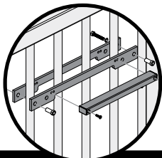
Mounting Plate for Guide Rail DCAC632----9004
