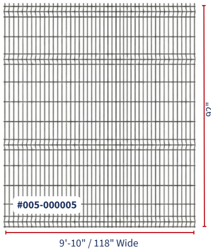
3D Fence 118" (W) x 8' (H)
