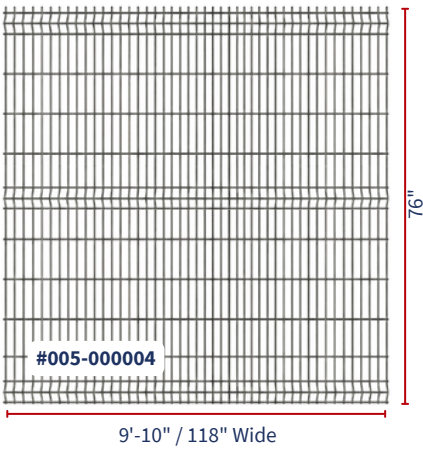
3D Fence 118" (W) x 6-1/2' (H)
