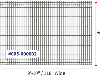
3D Fence 118" (W) x 5' (H)
