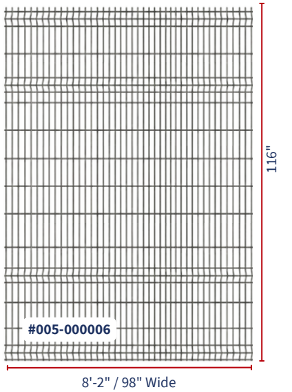
3D Fence 118" (W) x 10' (H)
