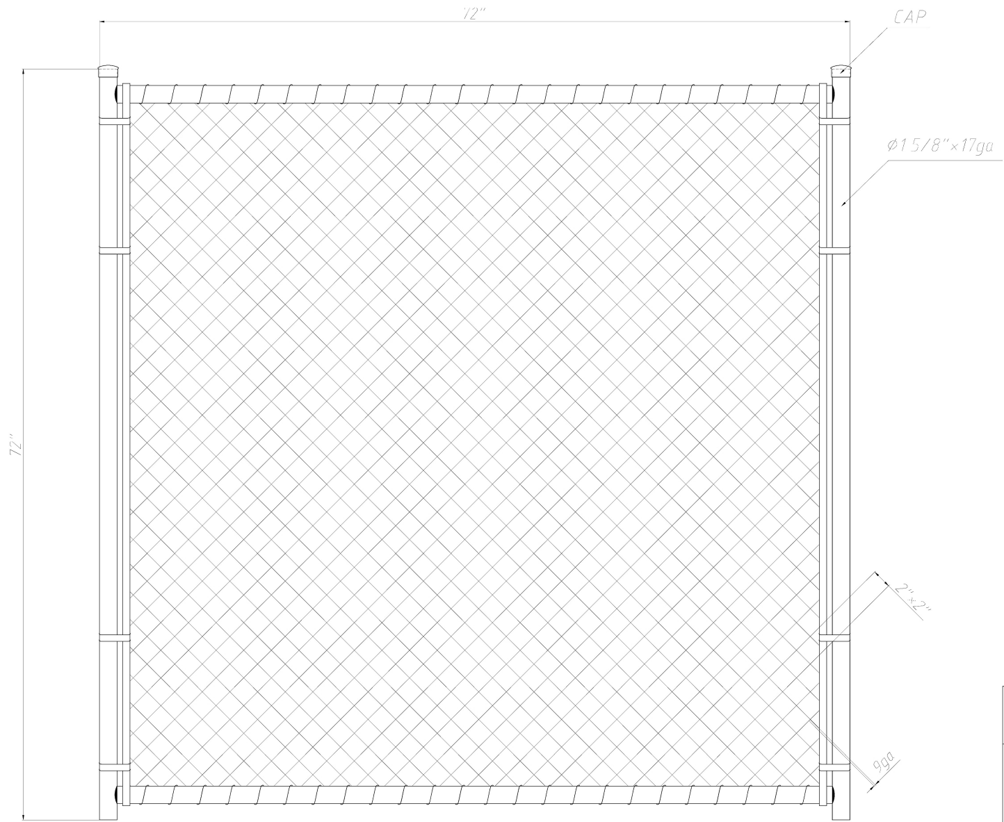
Commercial Walk Gate (No Posts) 72" Tall x 72" Wide
